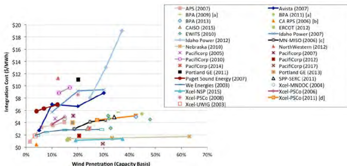
Figure 36 : US Dept of Energy 2016 Wind Technologies Market Report: Wind Integration Costs &amp; Penetration Levels
