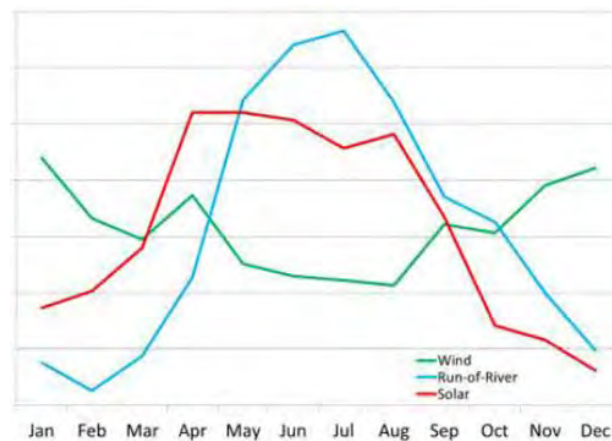
Figure 25: Monthly Energy Profile for Wind, Run-of-river and Solar
