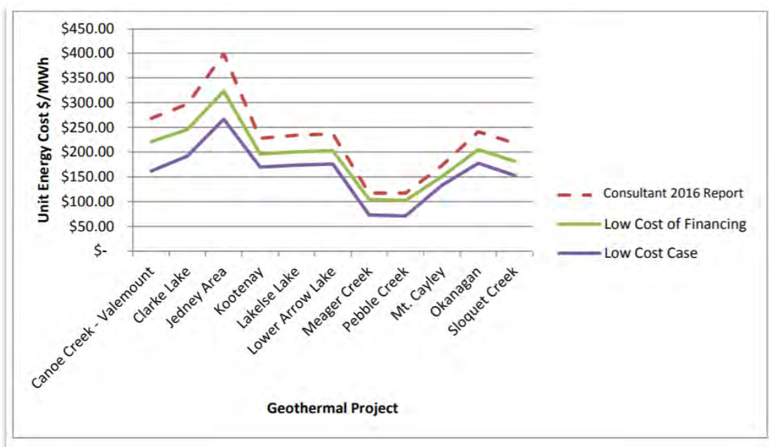
Figure 33: Geothermal Projects
